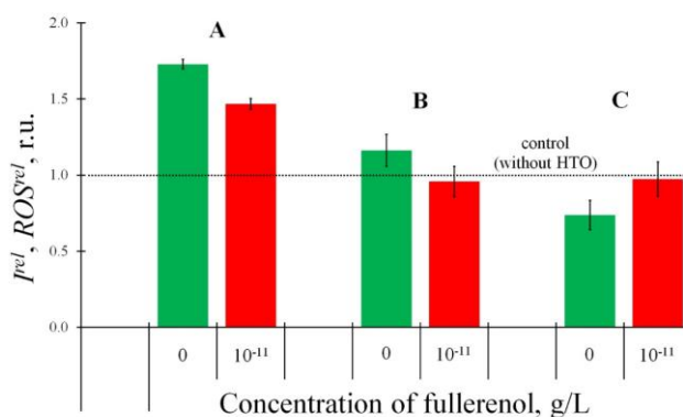
Figure 3. Relative luminescence intensity, I^{rel} , and ROS content, ROS^{rel} , in the absence and presence of fullerene, 10^{-11} g/L. Time of exposure was 4 h; HTO specific radioactivity was 500 MBq/L. (A) — bacterial luminescence, (B) — ROS content, (C) — luminescence of the enzyme system
